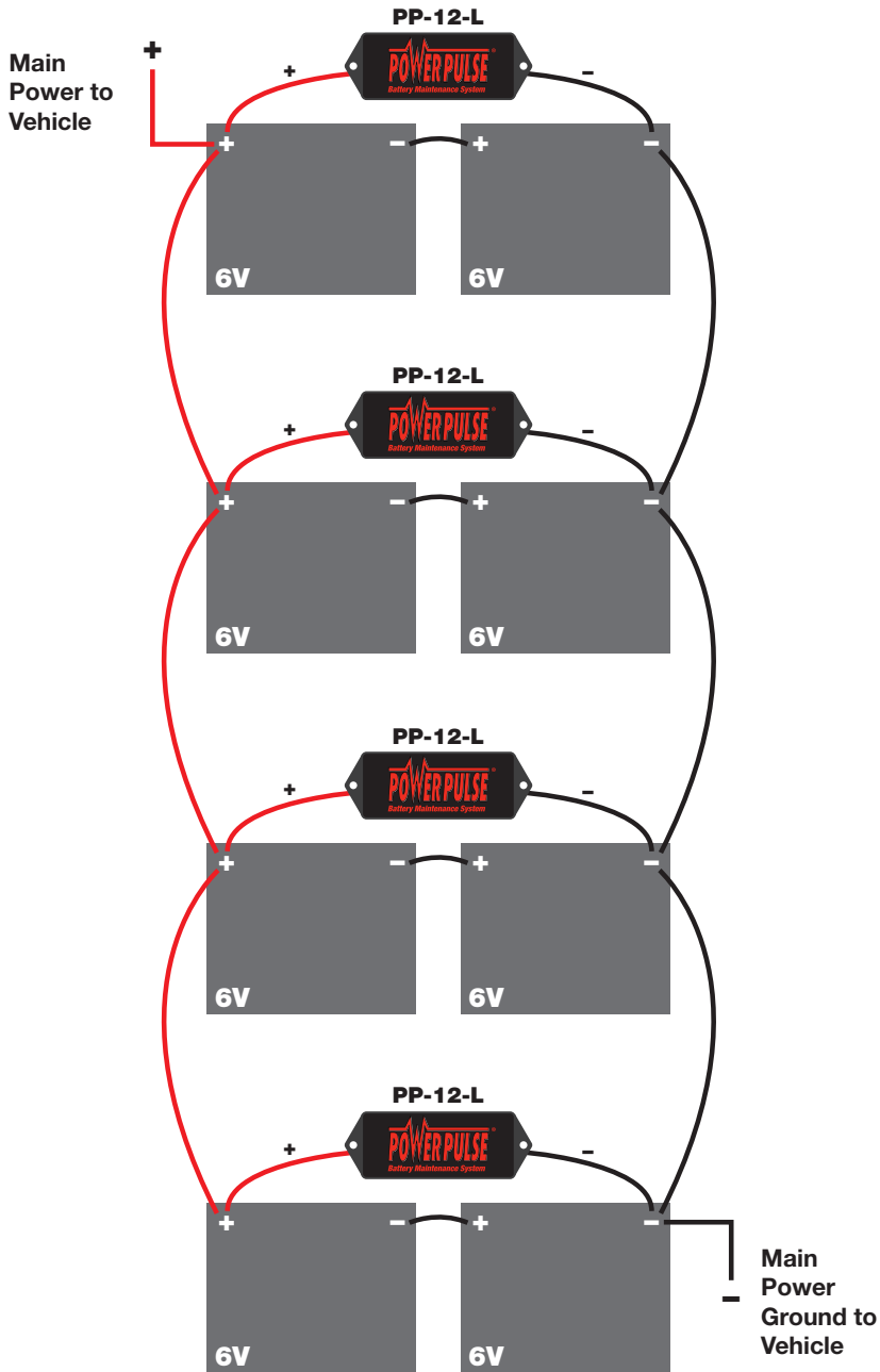
Multiple PP-12-L PowerPulse connection option with a 12V series/parallel connected 6V battery pack
