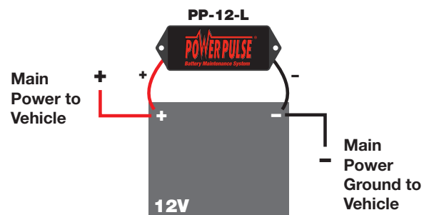
Single PP-12-L PowerPulse connection option with a single 12V battery
