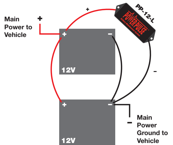
Single PP-12-L PowerPulse connection option with a 12V parallel connected 12V battery pack
